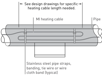
Figure 20 : Shoe and sleeve type support
