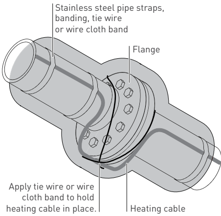
Figure 18: Flanges
