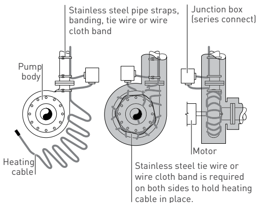
Figure 22: Pumps
