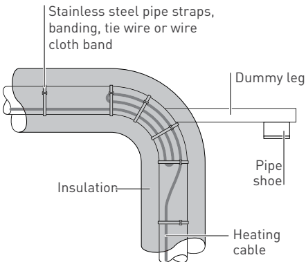
Figure 21: Dummy supports
